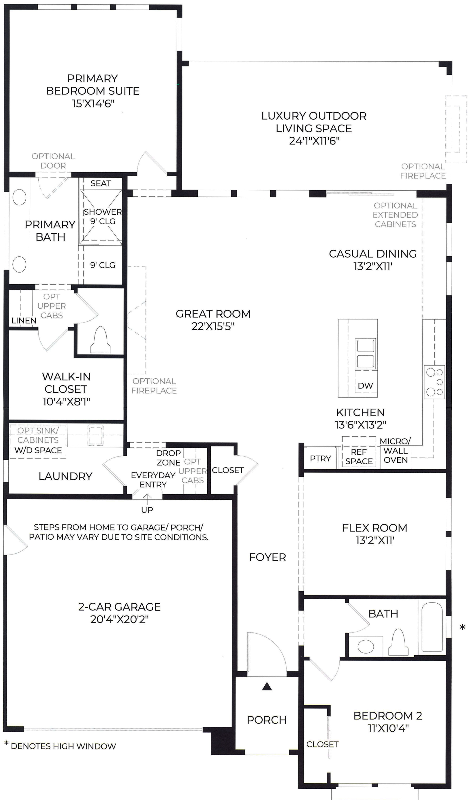
FLOOR PLAN 10' CEILING HEIGHT
