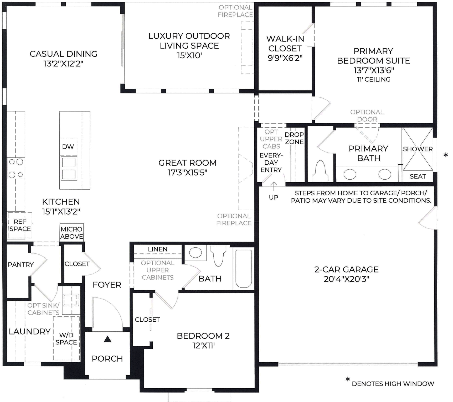
FLOOR PLAN 10' CEILING HEIGHT
